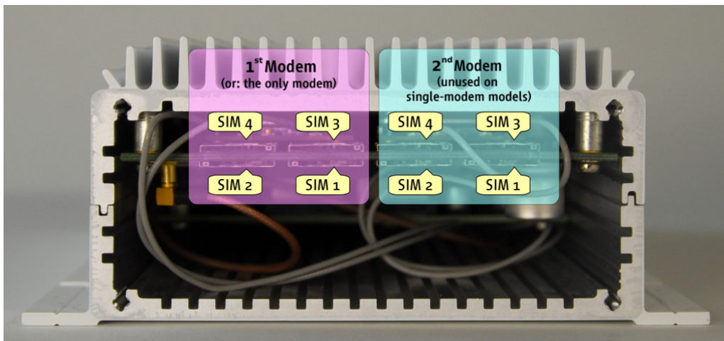
CyBox LTE 2 SIM Card Positions
