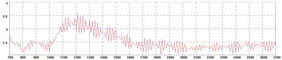
Typical VSWR (B4BE-7-27-5SP)
