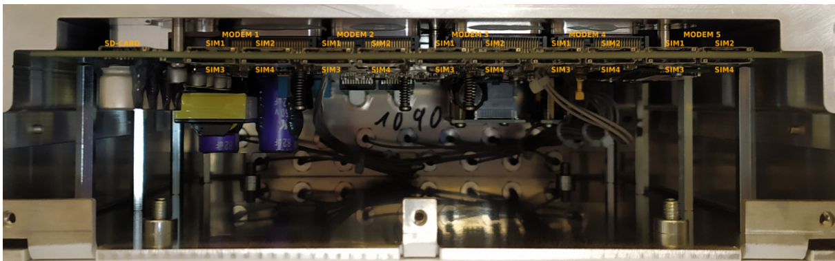
SIM slots on the CyBox GW
