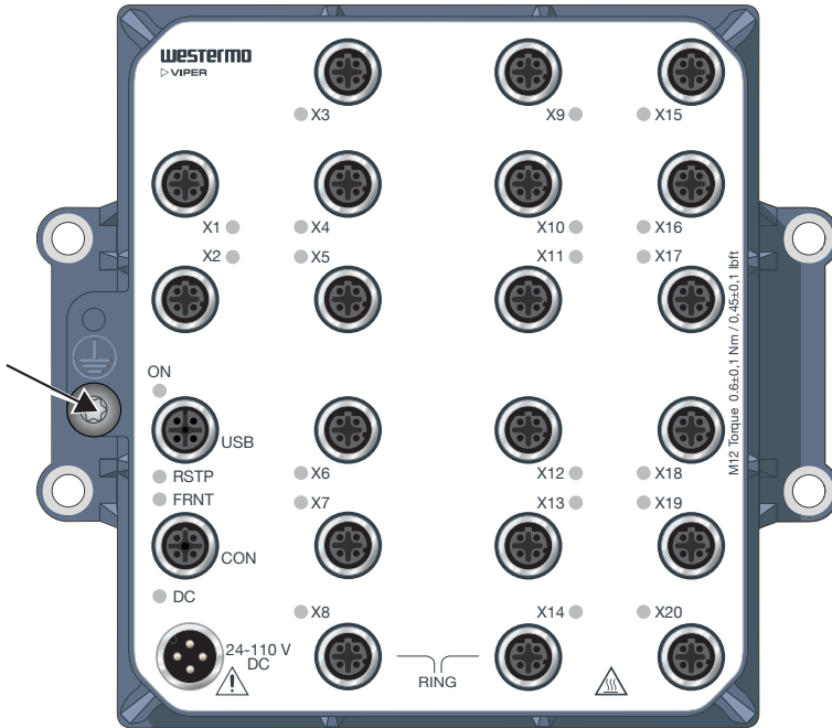
Figure 6. Earth connection
