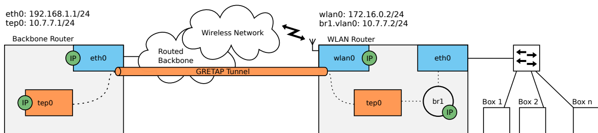
Figure 4.8: GRETAP in a Wireless Network
