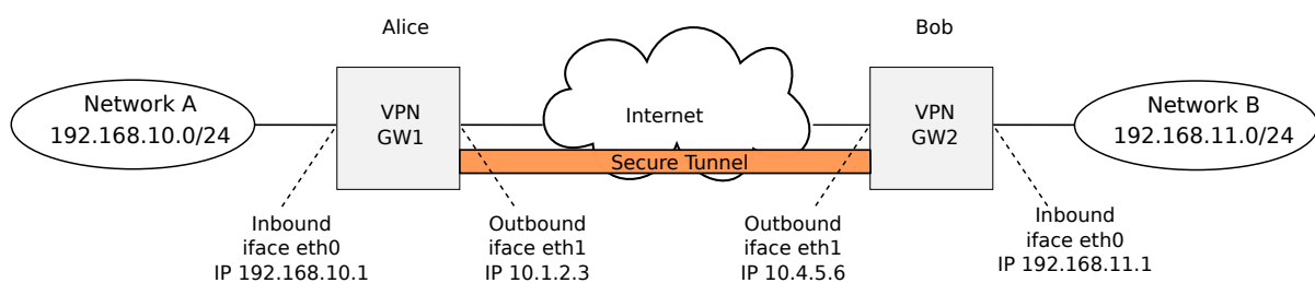
Figure 4.10: IPsec VPN Sample Topology
