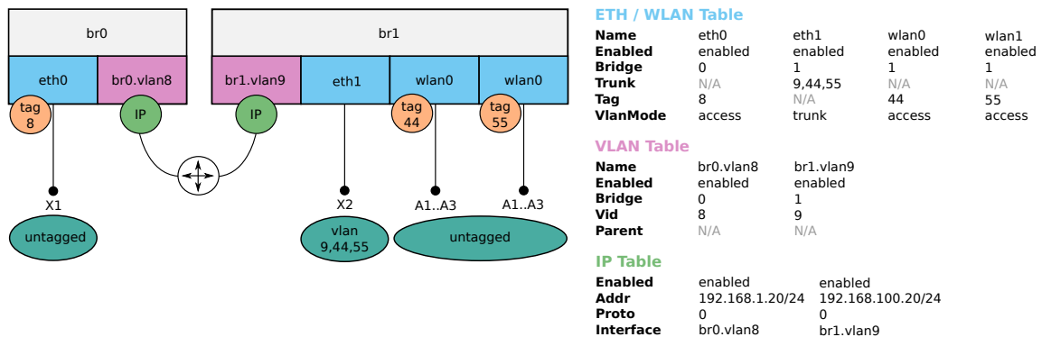
Figure 4.3: Access Point VLAN Network Configuration Example (Access Mode)
