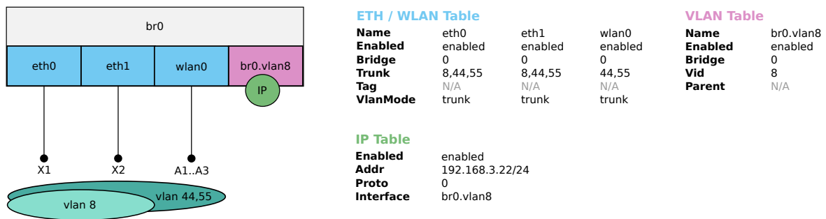
Figure 4.2: Access Point VLAN Network Configuration Example (Trunk Mode)
