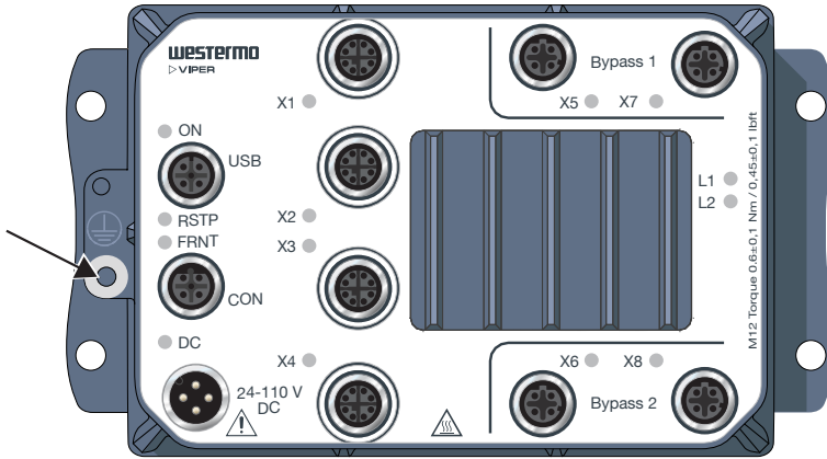
Figure 7. Earth connection
