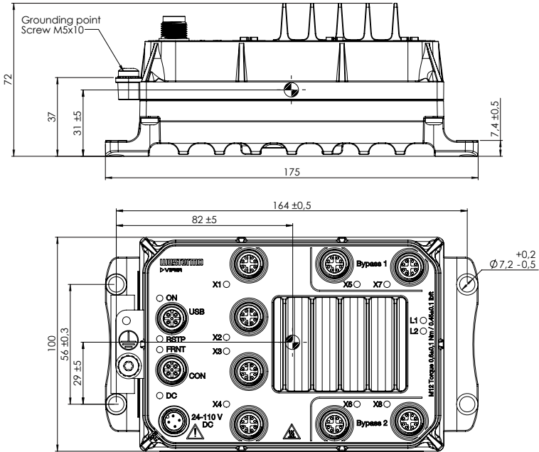
Figure 5. Dimensional drawing
