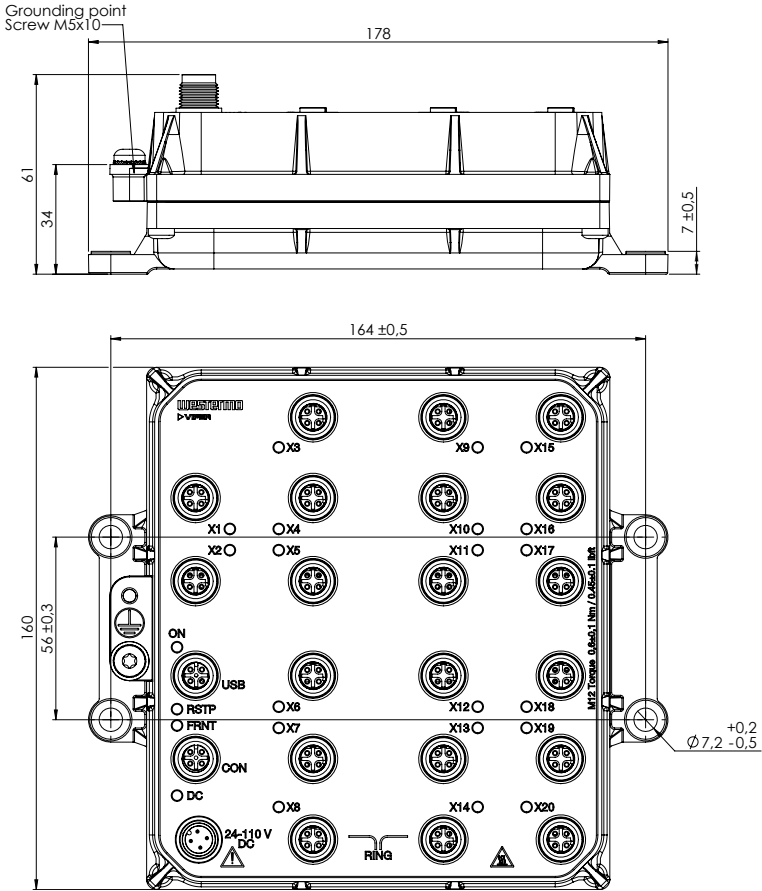
Figure 4. Dimensional drawing
