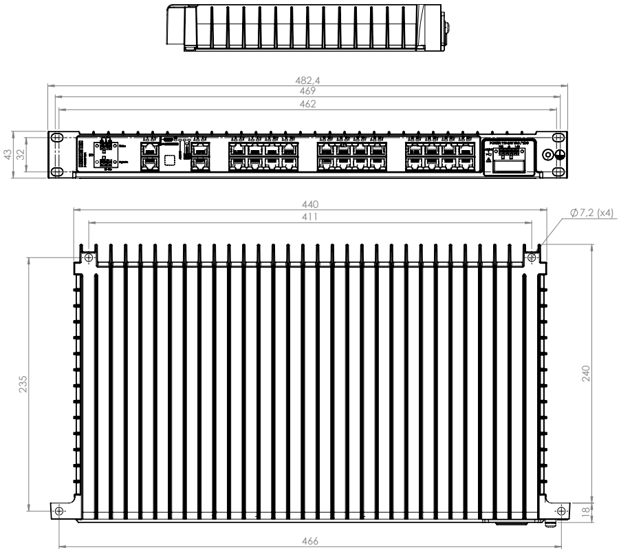
Figure 5. Dimensional drawing
