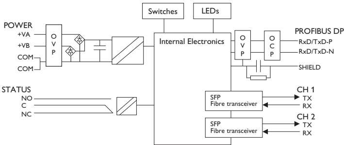
Figure 5. Block diagram for ODW-710-F2
