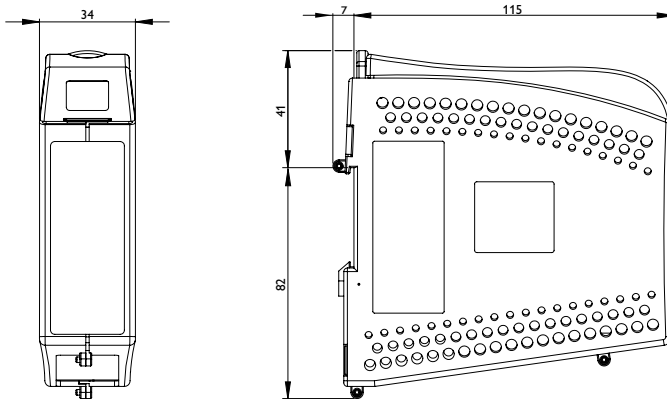
Figure 10. Dimensional drawing
