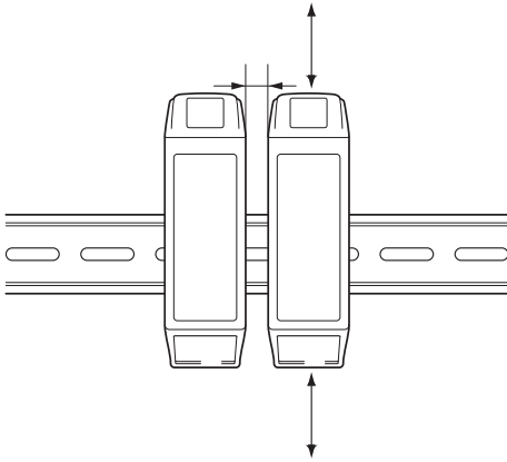
Figure 13. Minimum spacing of product
