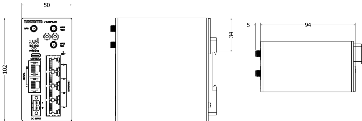
Figure 7. Dimensional drawing
