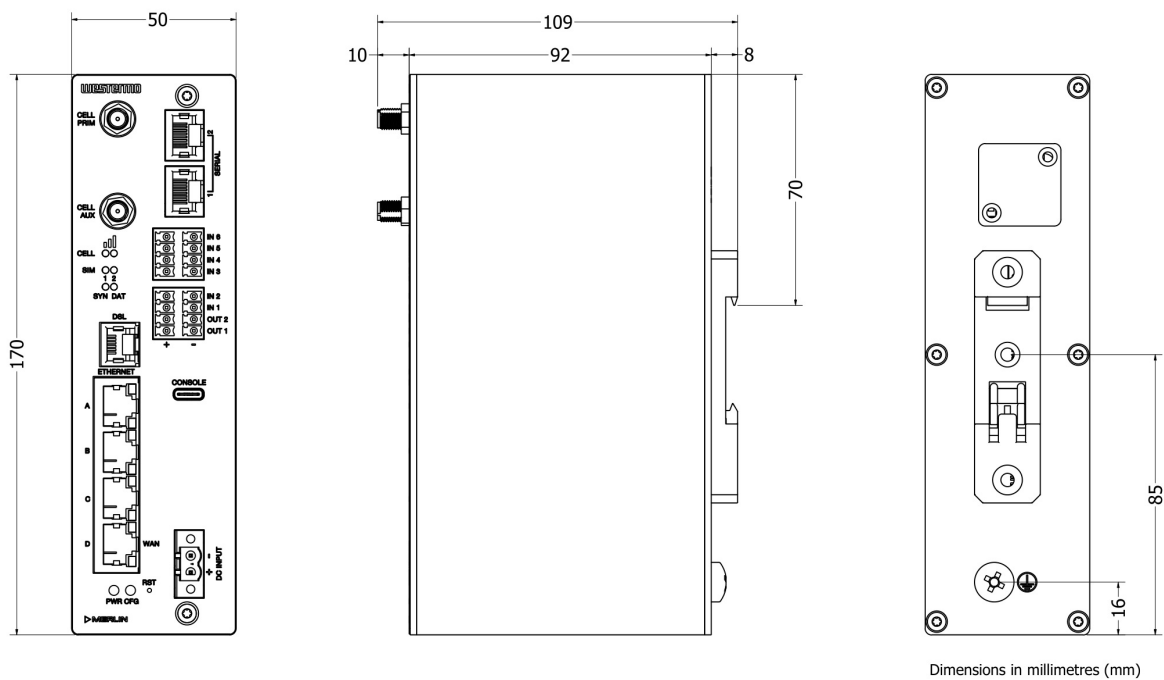
Figure 8. Dimensional drawing
